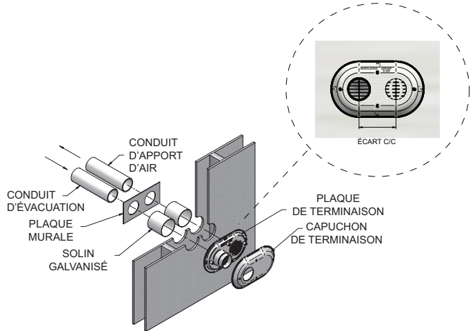
Figure 4-5A Terminaison murale
