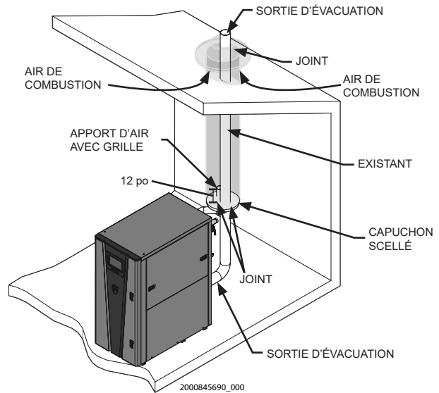
Figure 5-8 Ventilation concentrique, exemple 1
